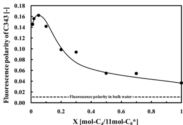
Fig. 9. Effect of the 1-butanol content on the fluorescence polarity of C343 in the W/O microemulsion. Measurement was carried out in PC=4.6 mM, W_{add} =10 and C343=3.56 \mu M.
